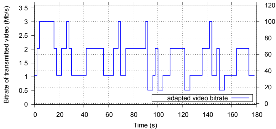
Figure 5: Quality adaptation with ZAAL for flow number 1 in ten concurrent flows test.
