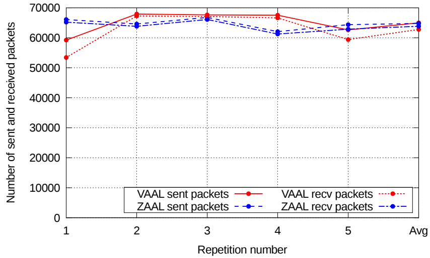
Figure 8: VAAL vs ZAAL in five concurrent flows test.
