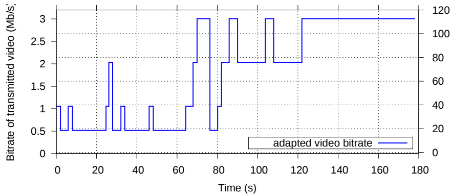
(b) with ZAAL: few zigzag occur
