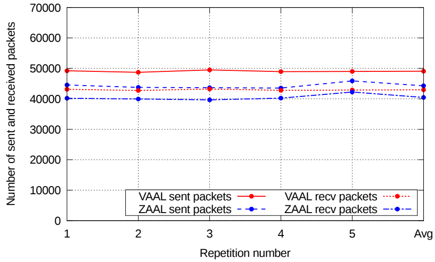
Figure 7: VAAL vs ZAAL in traffic shaping test.
