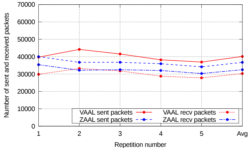
Figure 9: VAAL vs ZAAL in ten concurrent flows test.
