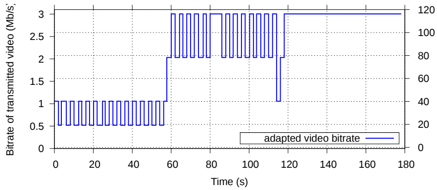
(a) without ZAAL: many zigzags occur
